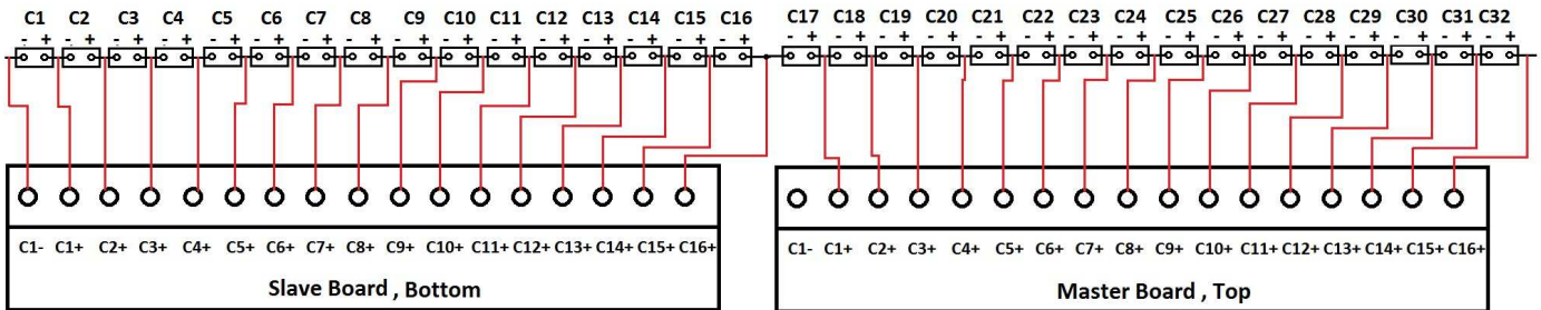
MiniBMS Centralized Installation Diagram
